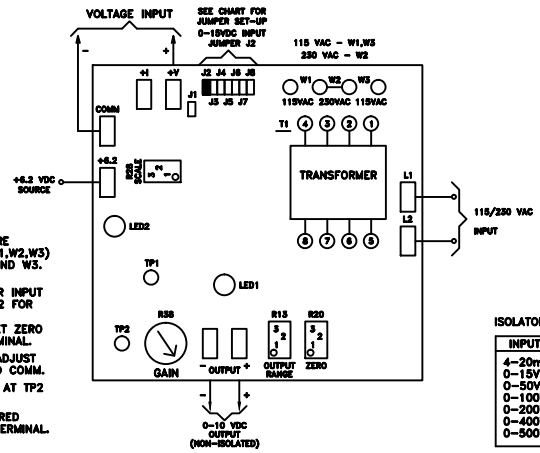
"EXTRON" #P1858-0210 ISOLATOR CARD 0-10 VDC - 0-10 VDC P.N. 274498 (DETAILS)
