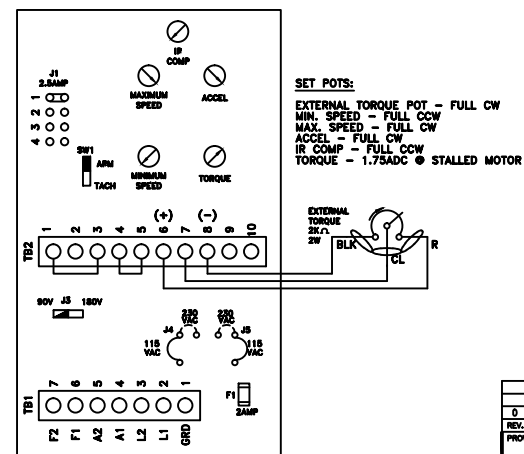
DETAILS OF "SECO-WARNER ELECTRIC" DC DRIVE "BRONCO II 1615"
